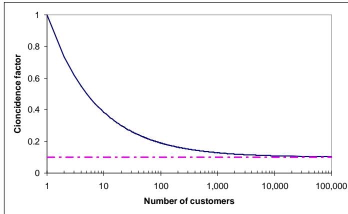
Figure 1: Load coincidence factor as a function of the number of typical households
